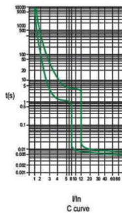
Standard B ( 4I_n < I < 6I_n ), C ( 8I_n < I < 12I_n );
