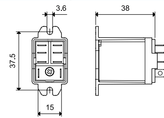
056.25 with relay
