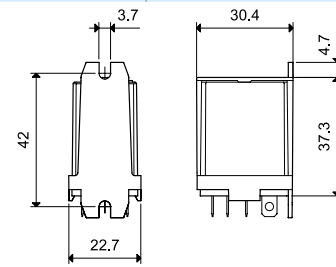
056.26 with relay
