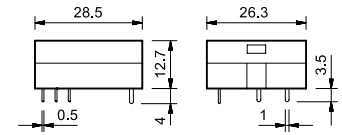
Type 40.11 (page 5)
