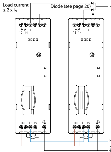
Parallel connection
