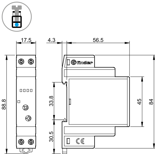
15.81 Screw terminal
