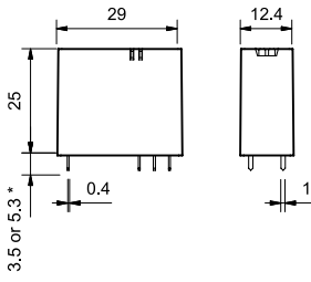
Type 40.31/51/52/61 (page 3)
