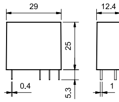
Type 40.31/51/52/61 (page 4)
