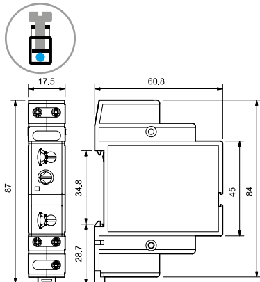
80.82 Screw terminal
