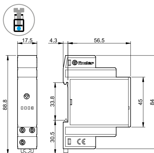
14.91 Screw terminal
