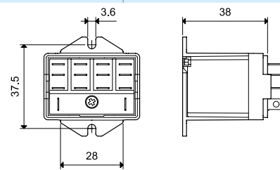
056.45 with relay
