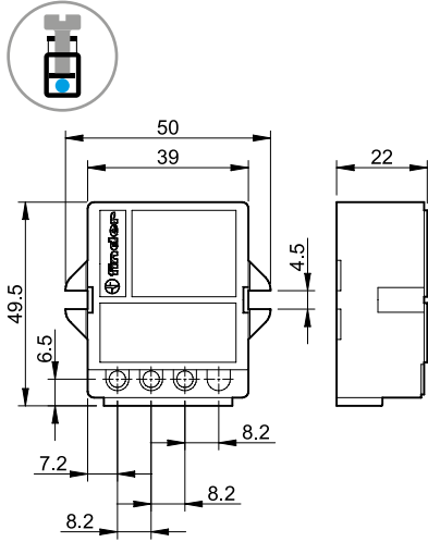
15.10 Screw terminal
