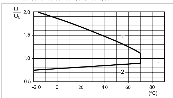
R 7S - AC coil operating range v ambient temperature - 7S.12/32 / 7S.23 / 7S.14/34 / 7S.16/36
