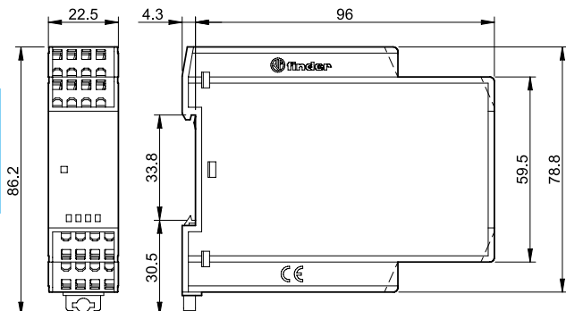
75.32 Screw terminal
