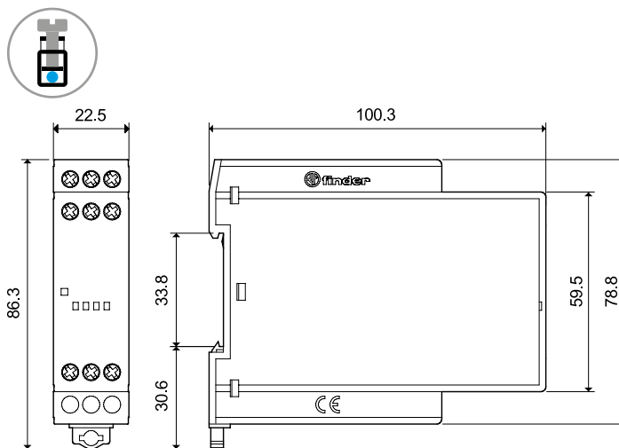
70.62 Screw terminal
