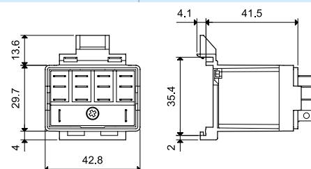
056.47 with relay
