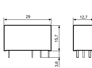
Type 41.52.6.xxx/41.61.6.xxx
