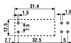
45.91...0310 (1 NO/SPST-NO)
