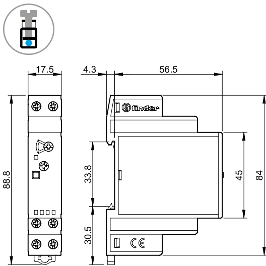
15.10 Screw terminal
