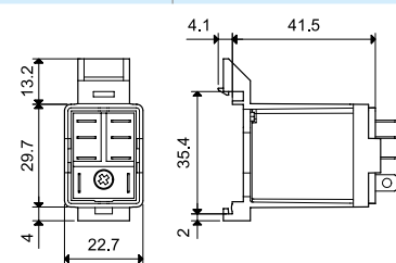
056.27 with relay
