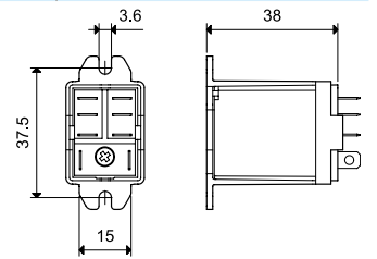
056.25 with relay
