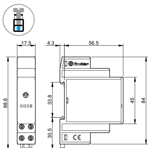
14.81 Screw terminal
