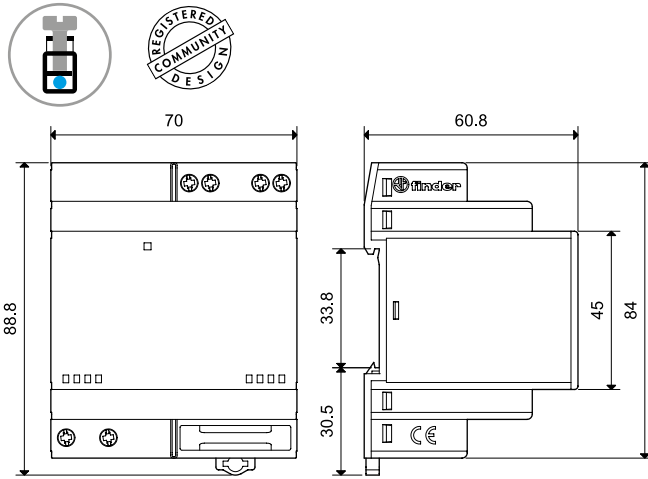
78.51 / 78.61 Screw terminal
