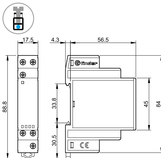
70.61 Screw terminal
