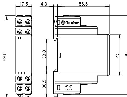
75.34 Screw terminal
