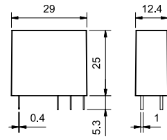
Type 40.31/51/52/61 (page 4)
