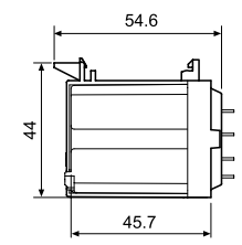
062.08 with relay
