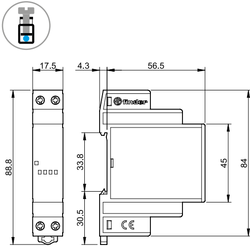
78.36 Screw terminal
