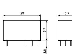
Type 41.52.6.xxx/41.61.6.xxx
