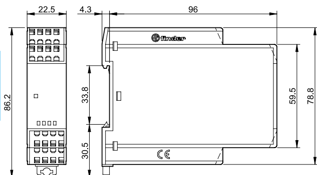
75.32 Screw terminal
