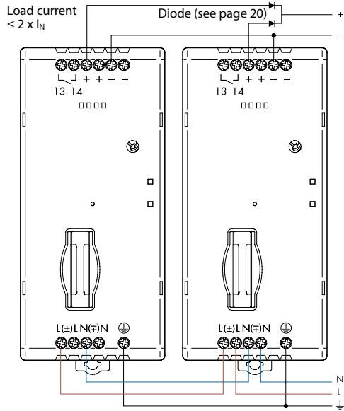
Parallel connection
