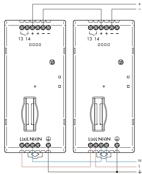
Series connection
