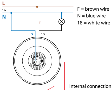
Type 10.61
