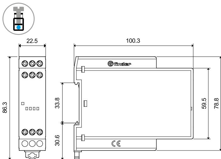
70.62 Screw terminal
