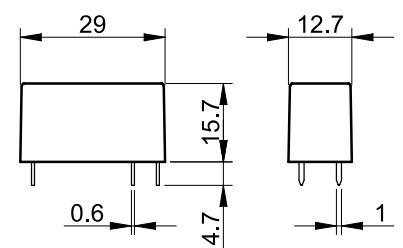
Type 41.81-9024/41.81-8240
