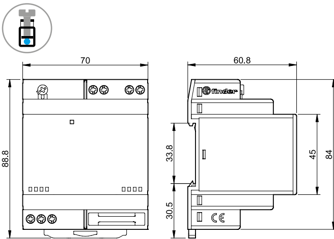
78.51 / 78.61 Screw terminal
