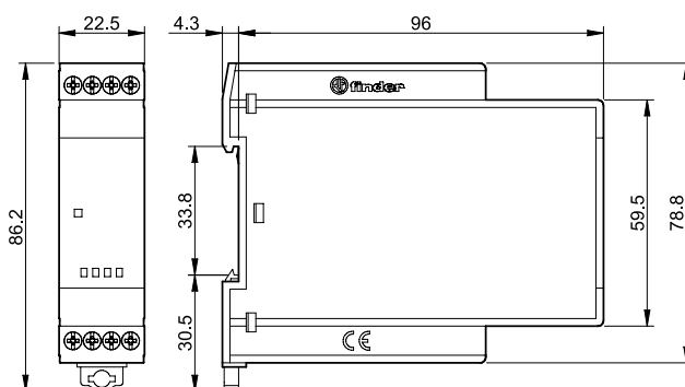
75.36 Screw terminal
