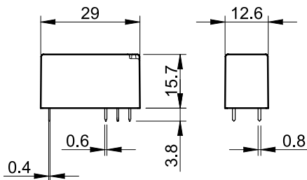
Type 41.31/52/61
