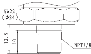
22: 1/8" NPT, Male, std. ANSI/ASME B1.20.1
