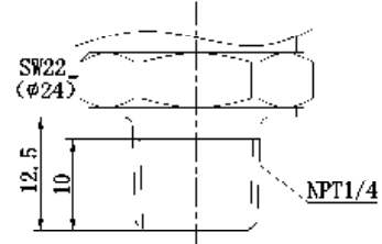
23: 1/4" NPT, Male, std. ANSI/ASME B1.20.1
